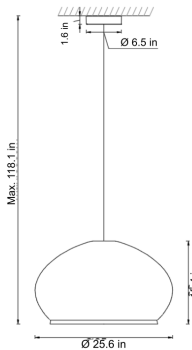
ARDEN LUME DIMENSIONS Vibinit - Model A - Large
