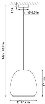
ARDEN LUME DIMENSIONS Vibinit - Model C
