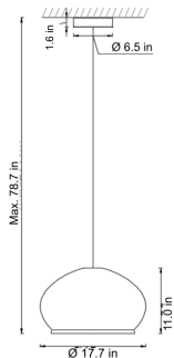
ARDEN LUME DIMENSIONS Vibinit - Model A - Small
