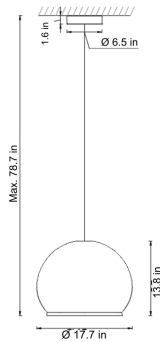
ARDEN LUME DIMENSIONS Vibinit - Model B - Small
