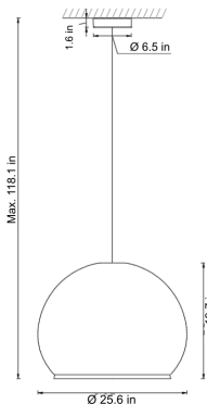
ARDEN LUME DIMENSIONS Vibinit - Model B - Large
